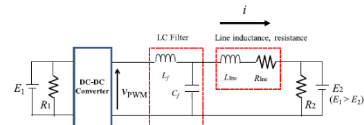
Fig. 1.Circuit for power flow control between two nodes.
